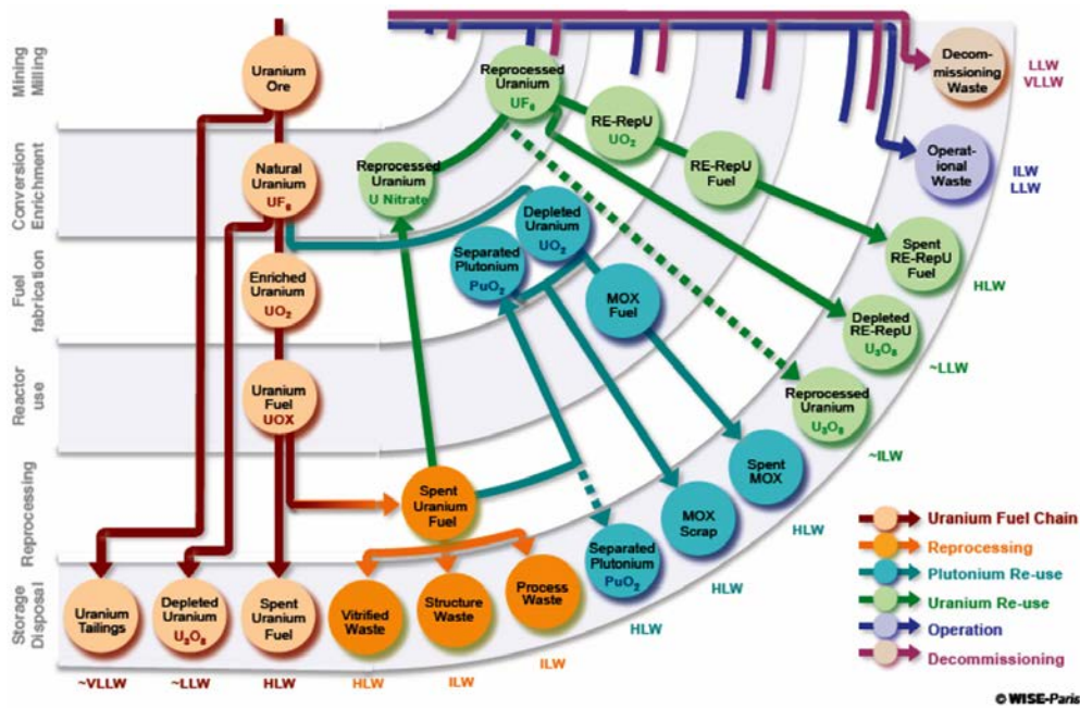
FIG. 5. Wastes and materials generated in the fuel chain [19]. (Courtesy of WISE-Paris.) HLW, high level waste; ILW, intermediate level waste; LLW, low level waste; MOX, mixed oxide; RE-RepU, re-enriched reprocessed uranium; UOX, uranium oxide; VLLW, very low level waste.
